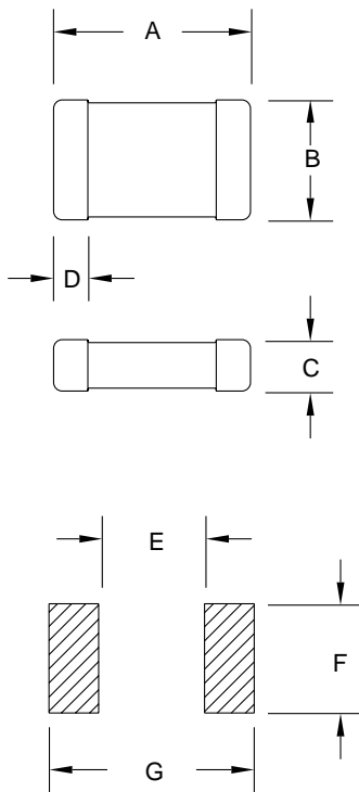
Pad Layout
